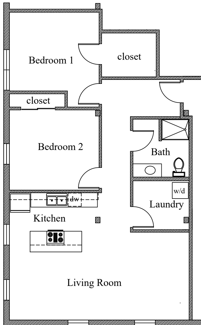
Apartment No. 4 : 1090 sq.ft. Scale: 1/8" = 1'-0"
